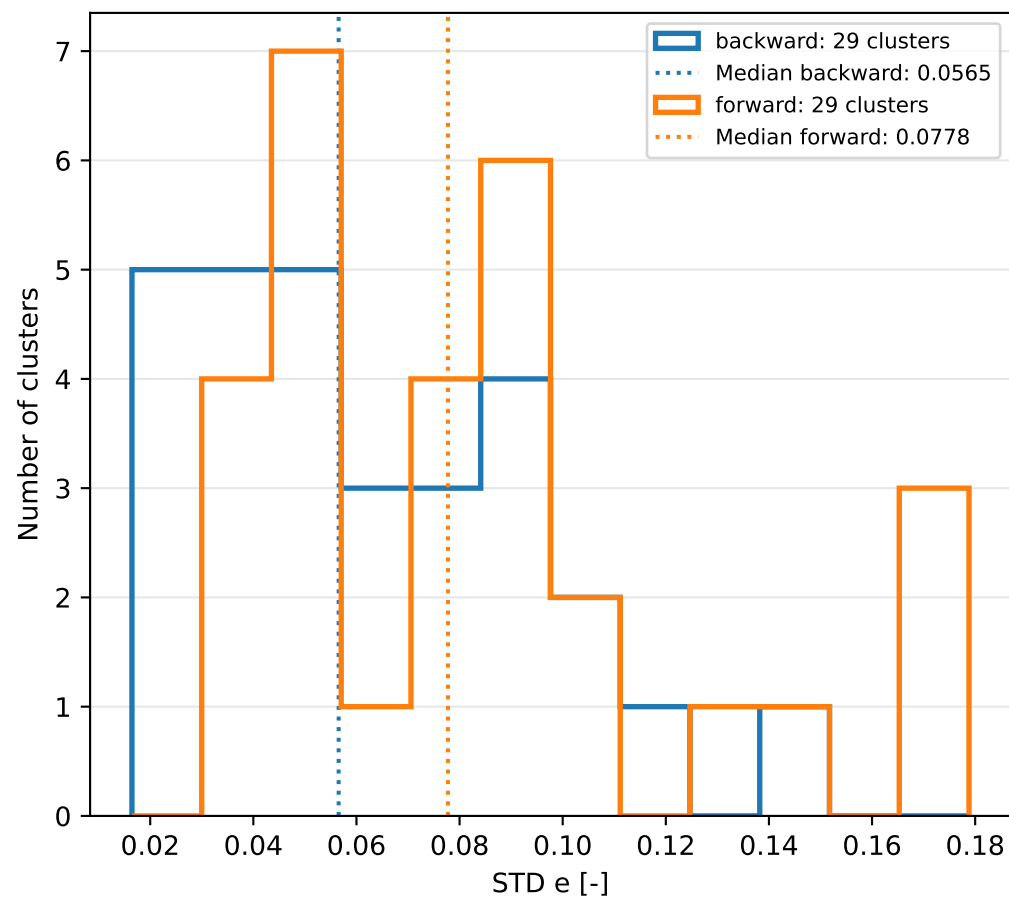
K=29 | Within-cluster STD distributions | Each cluster counts once
